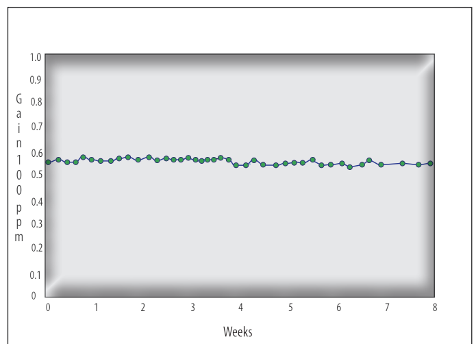
Humidity Response
